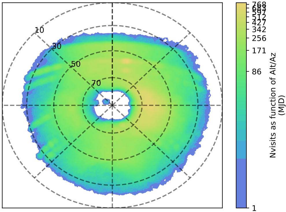
internal_u_expt30_nscale1.2v3.4_10yrs u: Nvisits as function of Alt/Az
