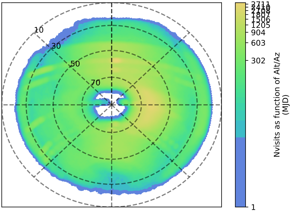
internal_u_expt30_nscale1.2v3.4_10yrs i: Nvisits as function of Alt/Az
