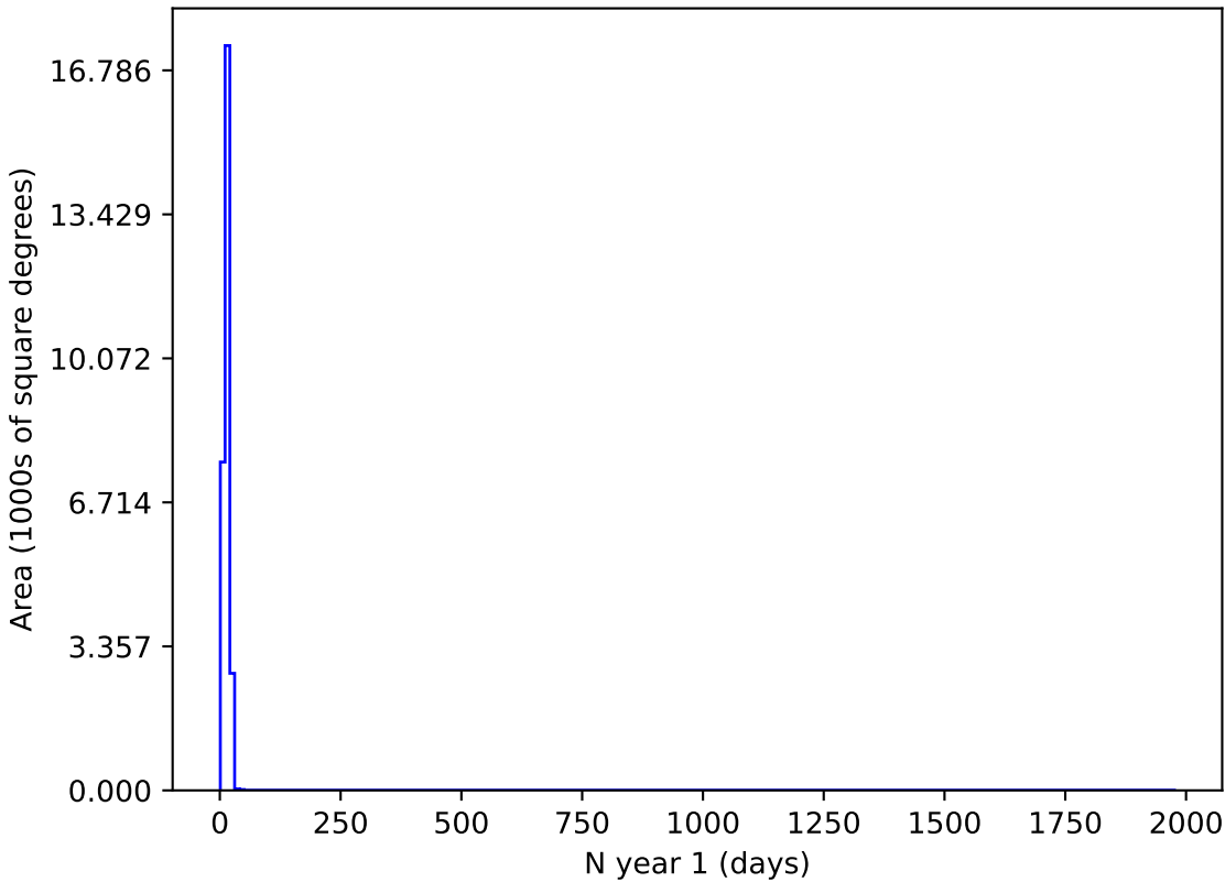
internal_u_expt30_nscale1.2v3.4_10yrs z and night < 365: N year 1
