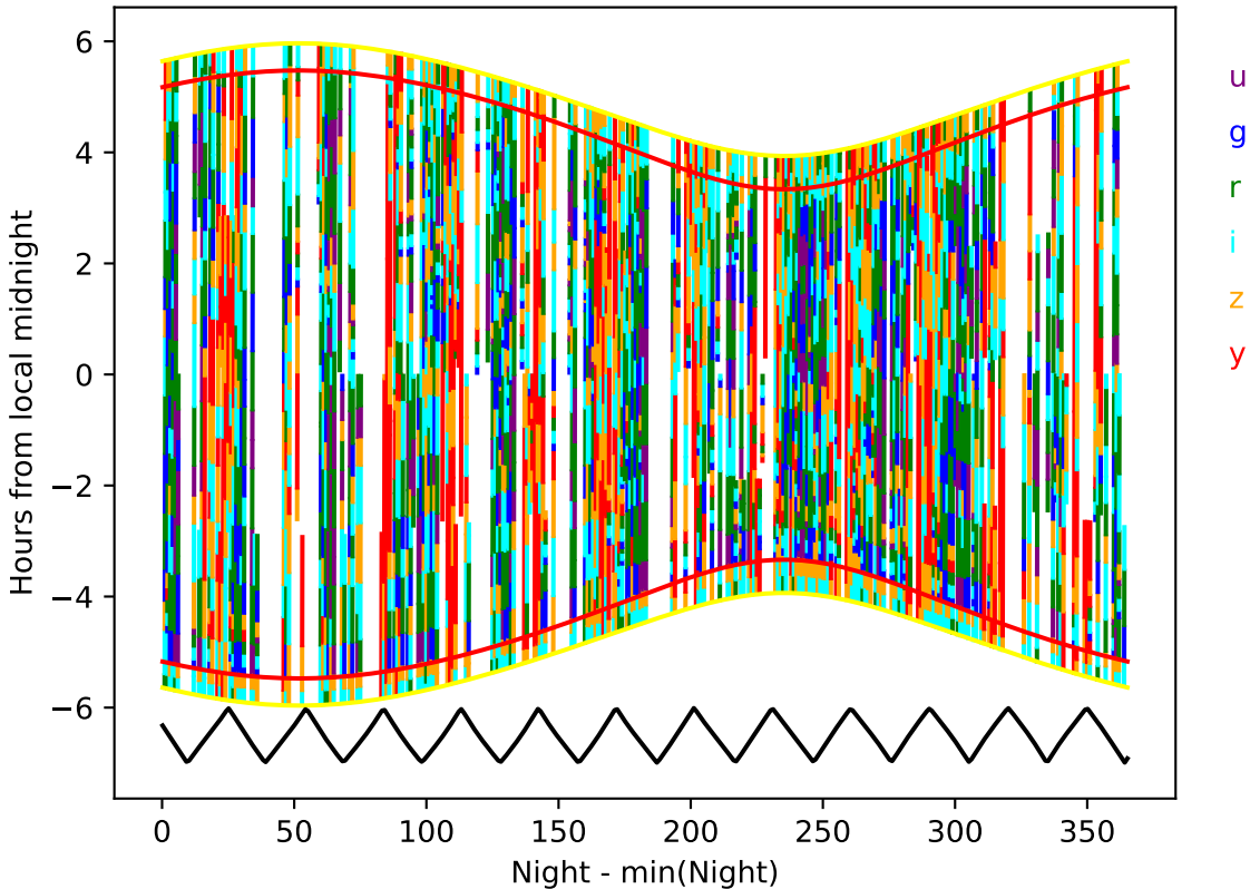
internal_u_expt30_nscale1.2v3.4_10yrs year 7-8: Hourglass
