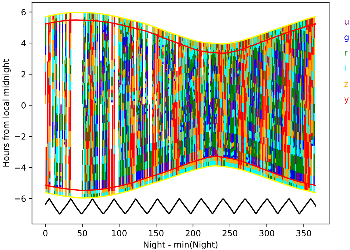
internal_u_expt30_nscale1.2v3.4_10yrs year 6-7: Hourglass
