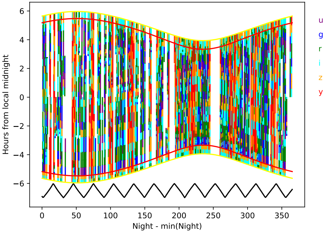
internal_u_expt30_nscale1.2v3.4_10yrs year 5-6: Hourglass
