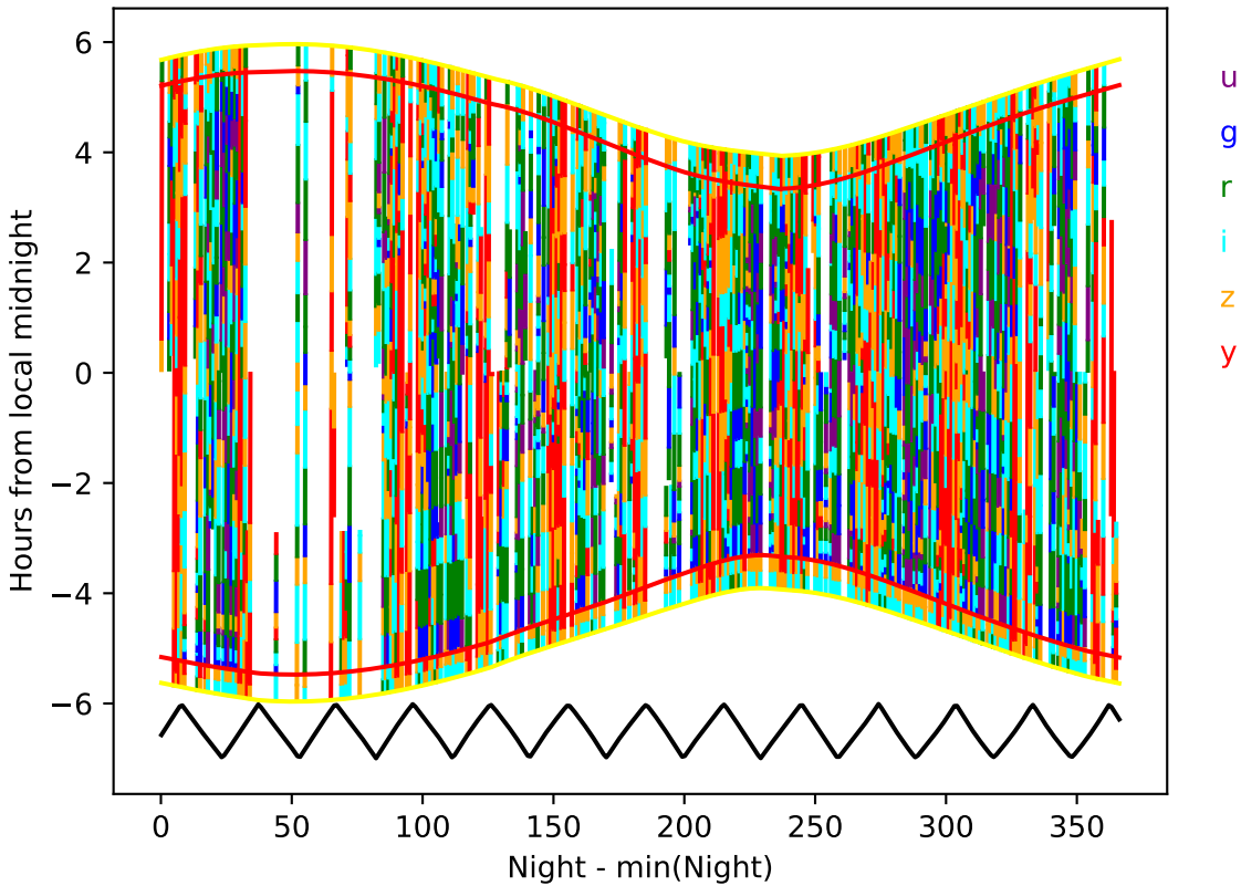
internal_u_expt30_nscale1.2v3.4_10yrs year 3-4: Hourglass
