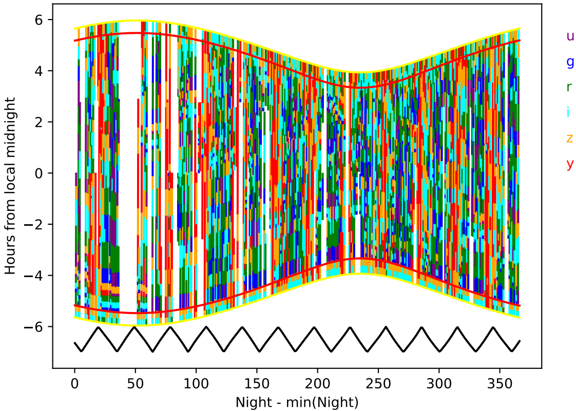
internal_u_expt30_nscale1.2v3.4_10yrs year 2-3: Hourglass
