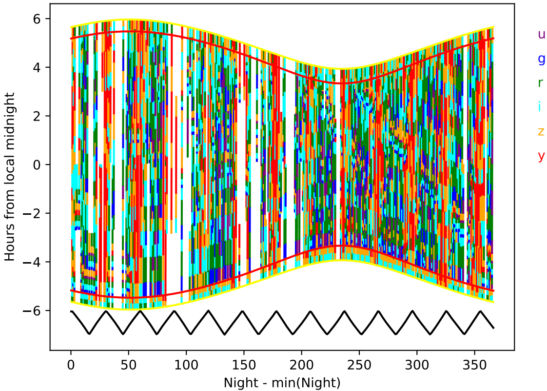
internal_u_expt30_nscale1.2v3.4_10yrs year 1-2: Hourglass
