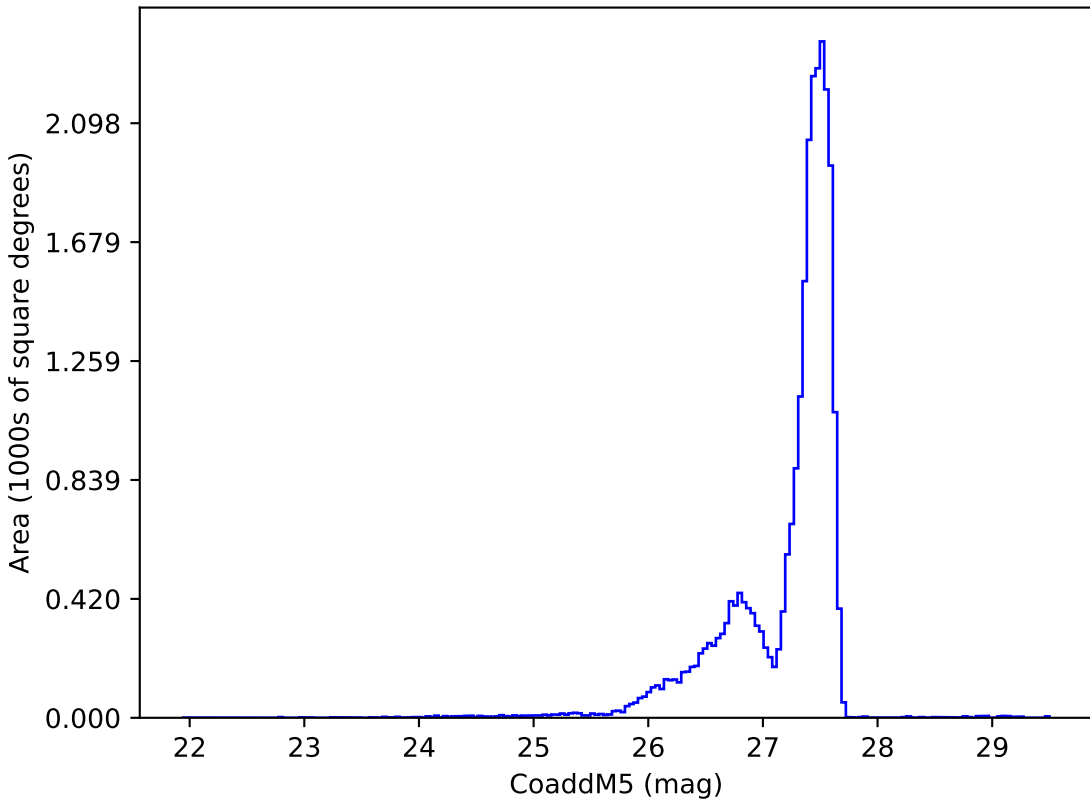
internal_u_expt30_nscale1.2v3.4_10yrs : CoaddM5
