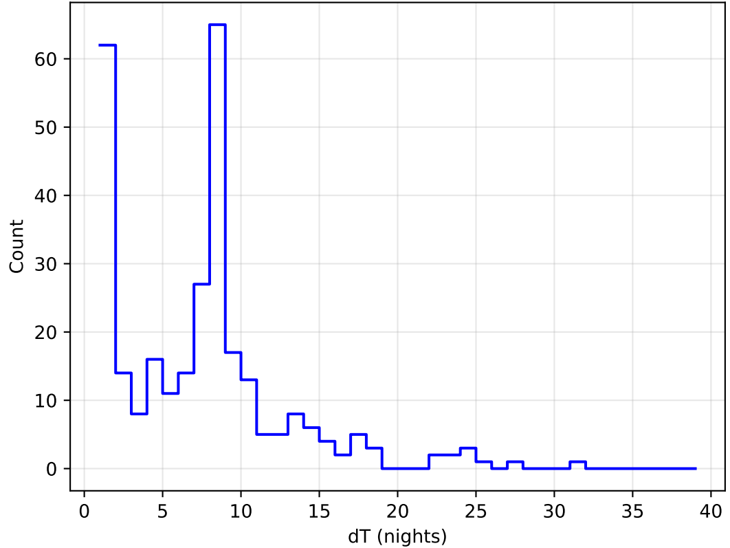
internal_u_expt30_nscale1.2v3.4_10yrs all bands: DD:XMM_LSS Delta Nights Histogram
