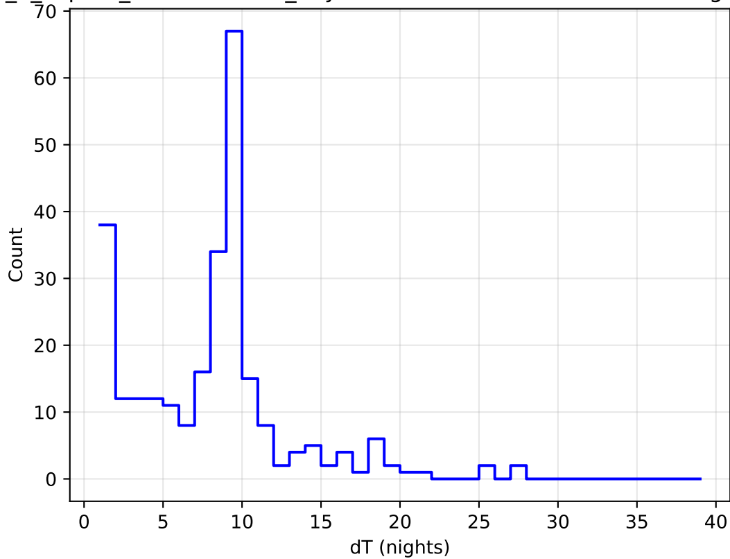
internal_u_expt30_nscale1.2v3.4_10yrs all bands: DD:ELAISS1 Delta Nights Histogram
