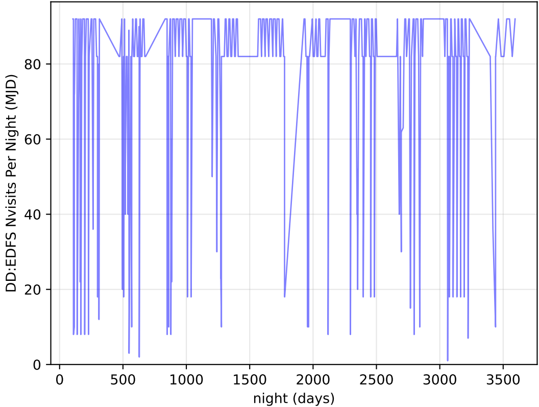
internal_u_expt30_nscale1.2v3.4_10yrs all bands: DD:EDFS Nvisits Per Night
