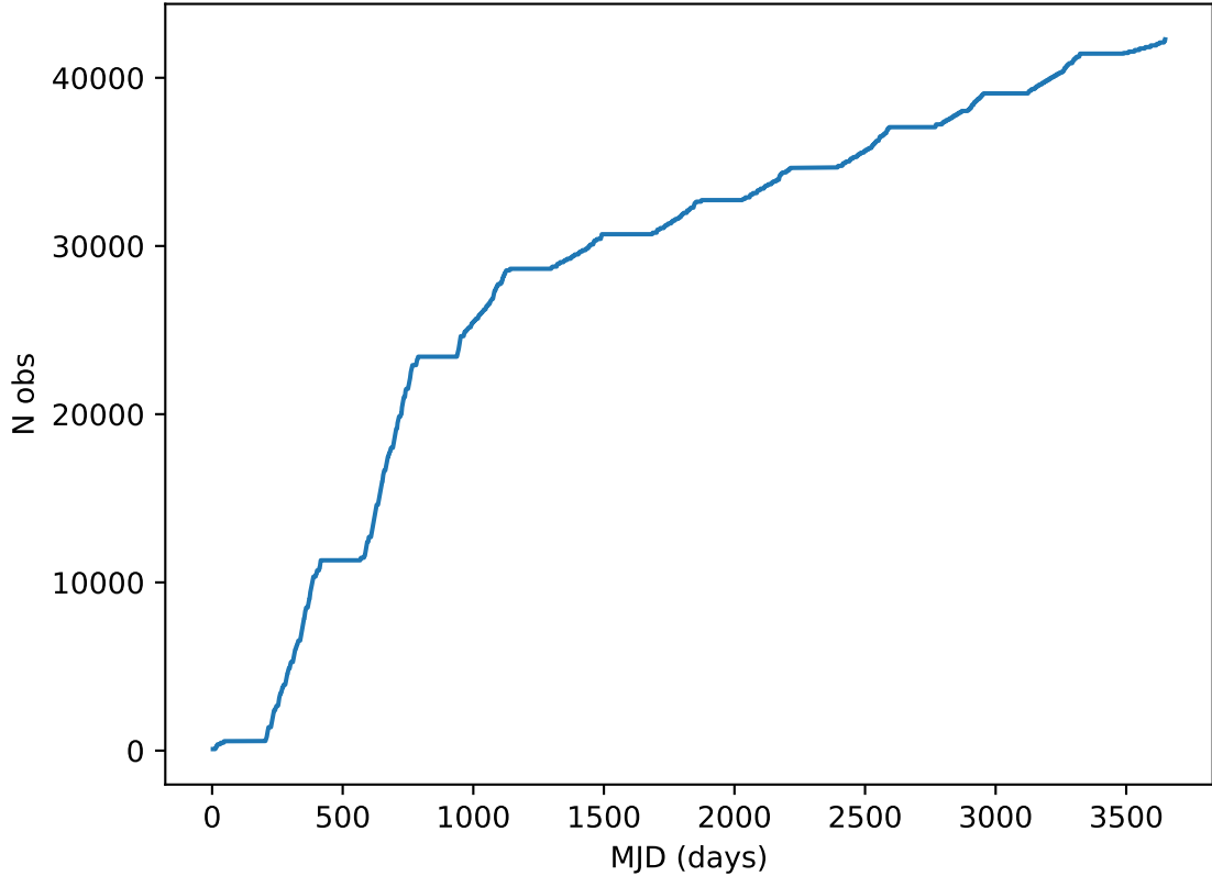
internal_u_expt30_nscale1.2v3.4_10yrs all bands: DD: COSMOS Cumulative NVisits
