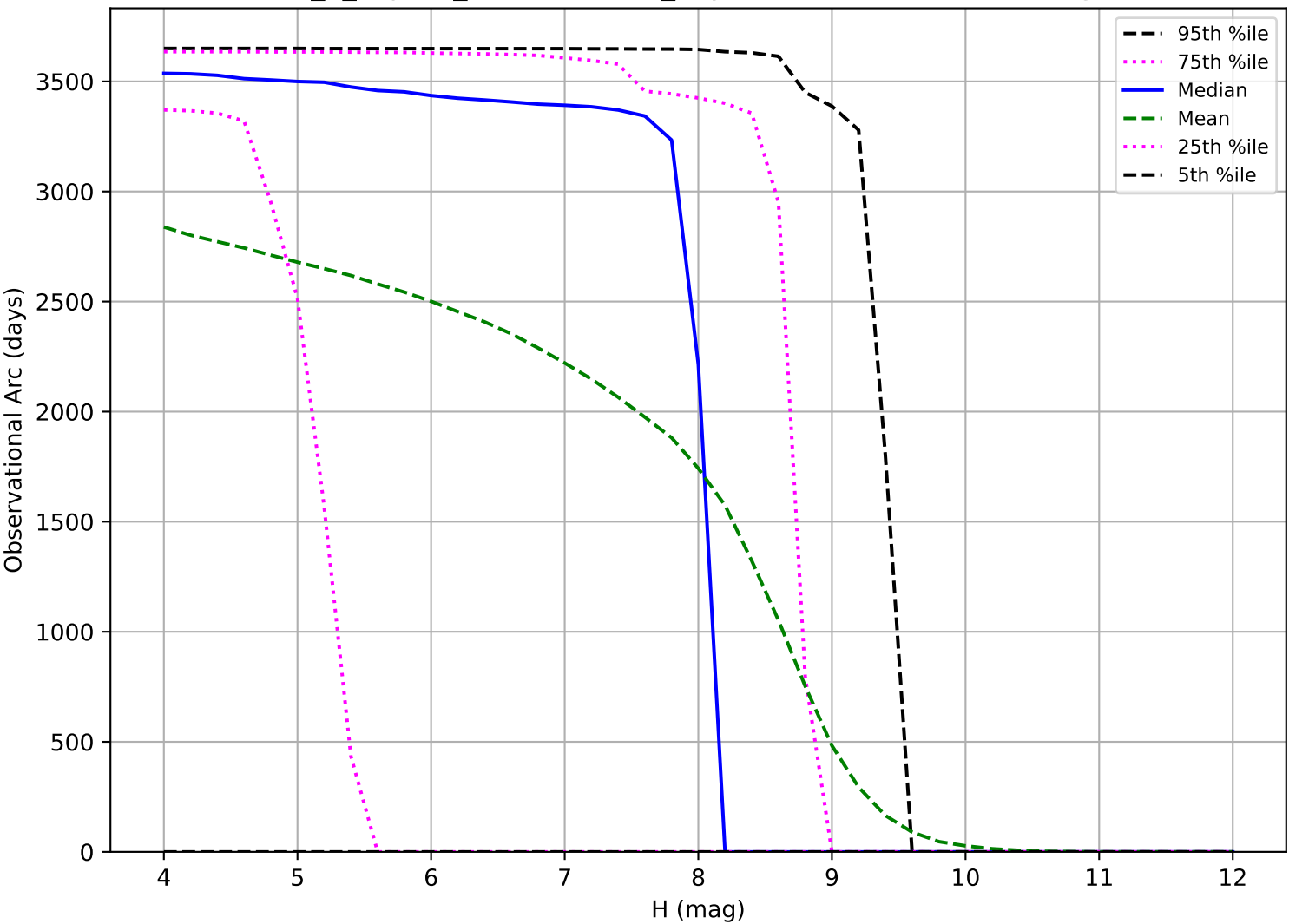
internal_u_expt30_nscale1.1v3.4_10yrs: Observational Arc Length TNO
