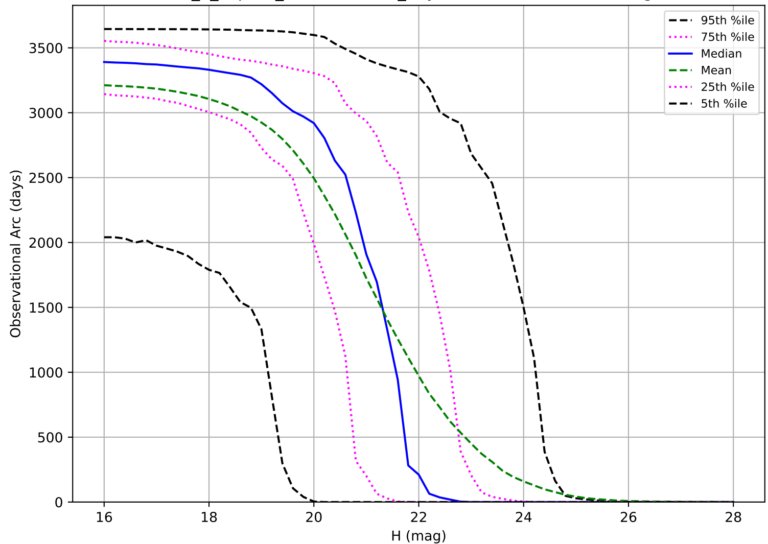
internal_u_expt30_nscale1.1v3.4_10yrs: Observational Arc Length PHA
