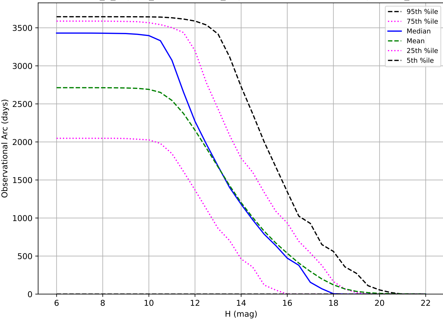
internal_u_expt30_nscale1.1v3.4_10yrs: Observational Arc Length OCC_r5
