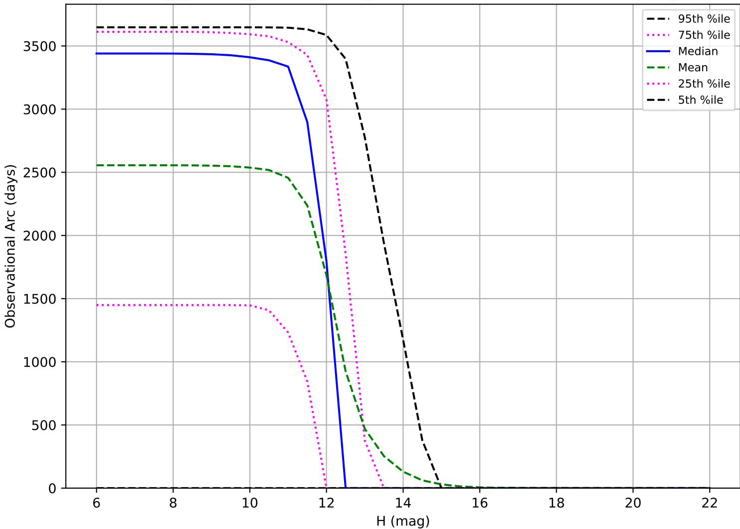
internal_u_expt30_nscale1.1v3.4_10yrs: Observational Arc Length OCC_r20
