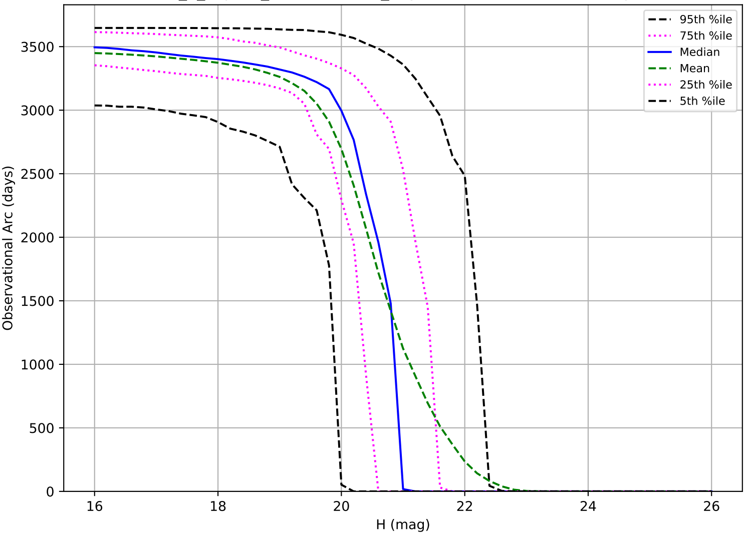
internal_u_expt30_nscale1.1v3.4_10yrs: Observational Arc Length MBA
