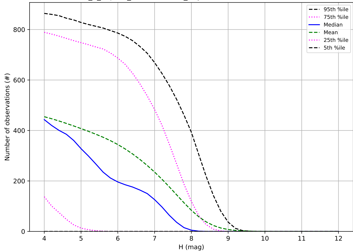
internal_u_expt30_nscale1.1v3.4_10yrs: Number of observations TNO
