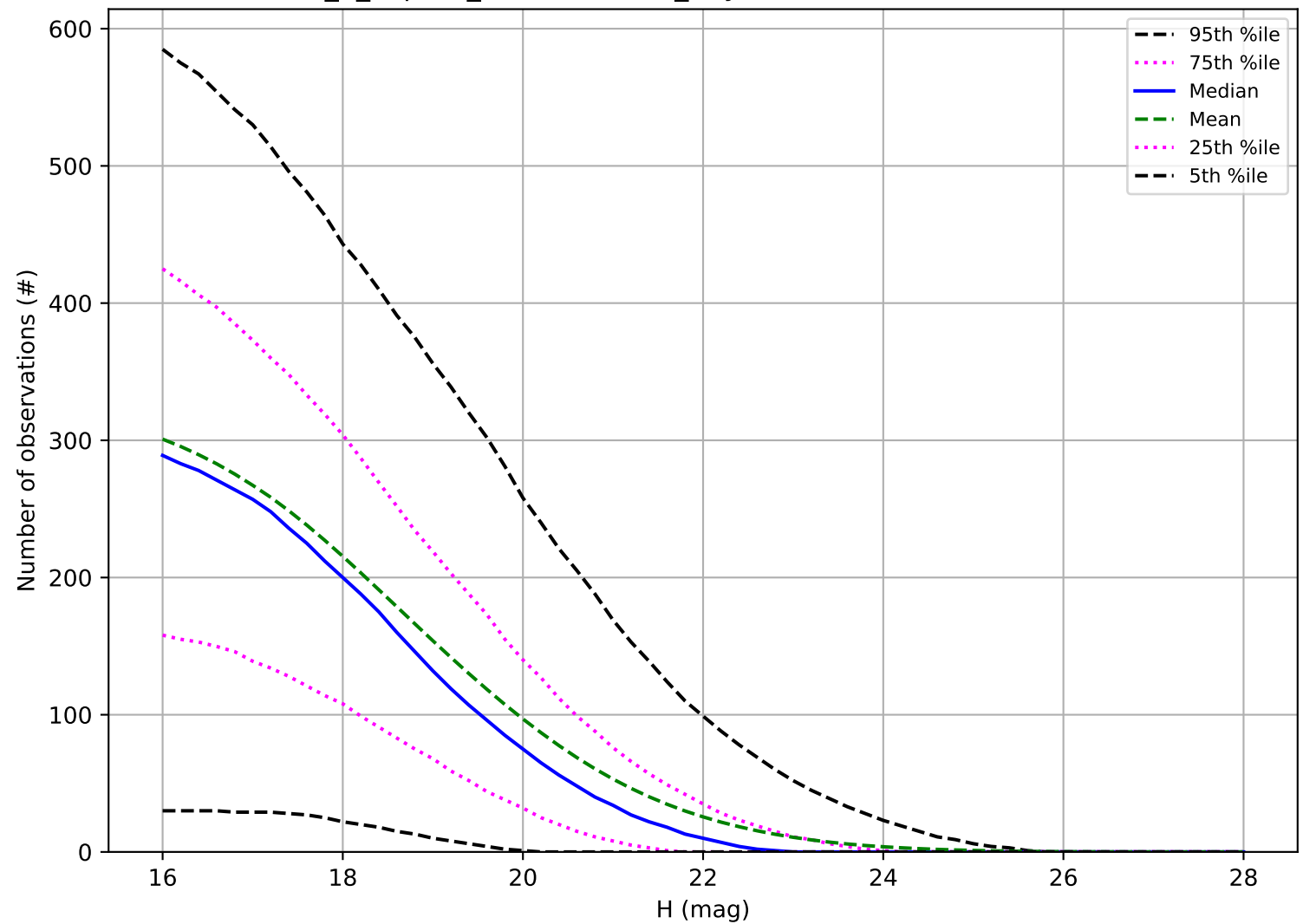
internal_u_expt30_nscale1.1v3.4_10yrs: Number of observations NEO
