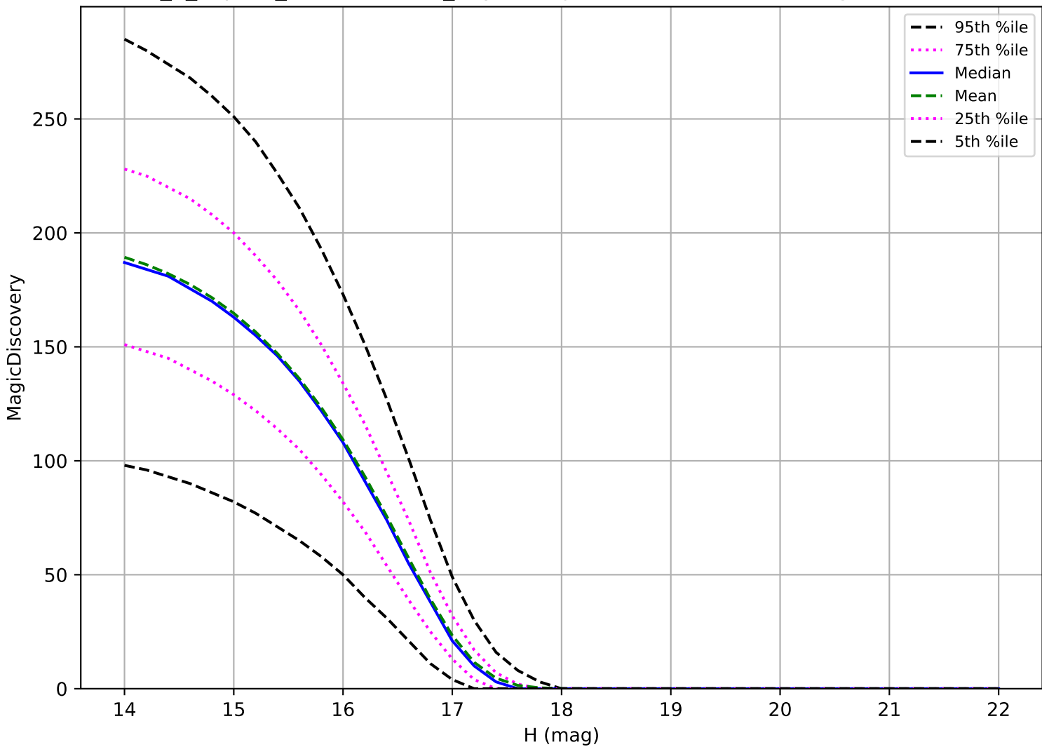
internal_u_expt30_nscale1.1v3.4_10yrs: Trojan 6 detections in 60 nights detection loss
