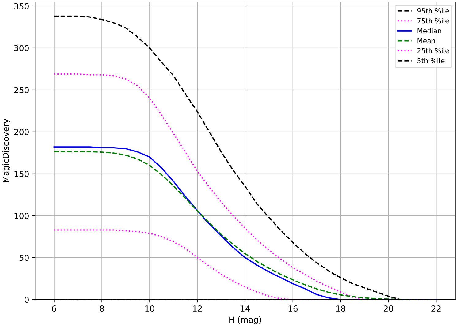
internal_u_expt30_nscale1.1v3.4_10yrs: OCC_r5 6 detections in 60 nights detection loss
