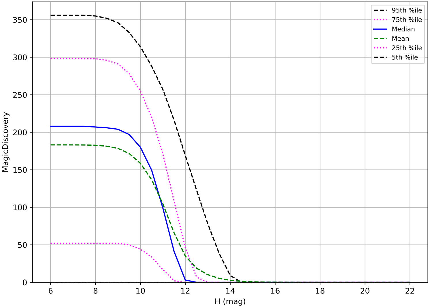
internal_u_expt30_nscale1.1v3.4_10yrs: OCC_r20 6 detections in 60 nights detection loss
