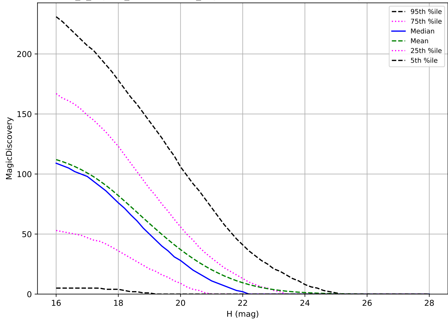
internal_u_expt30_nscale1.1v3.4_10yrs: NEO 6 detections in 60 nights detection loss
