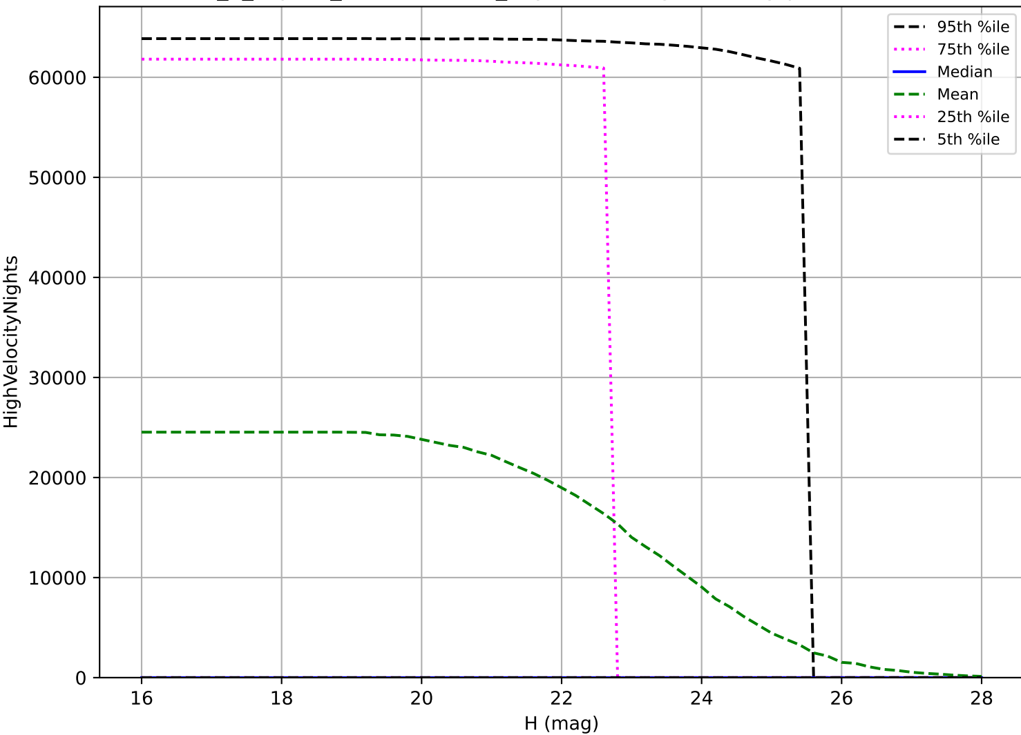
internal_u_expt30_nscale1.1v3.4_10yrs: PHA High velocity pair detection loss
