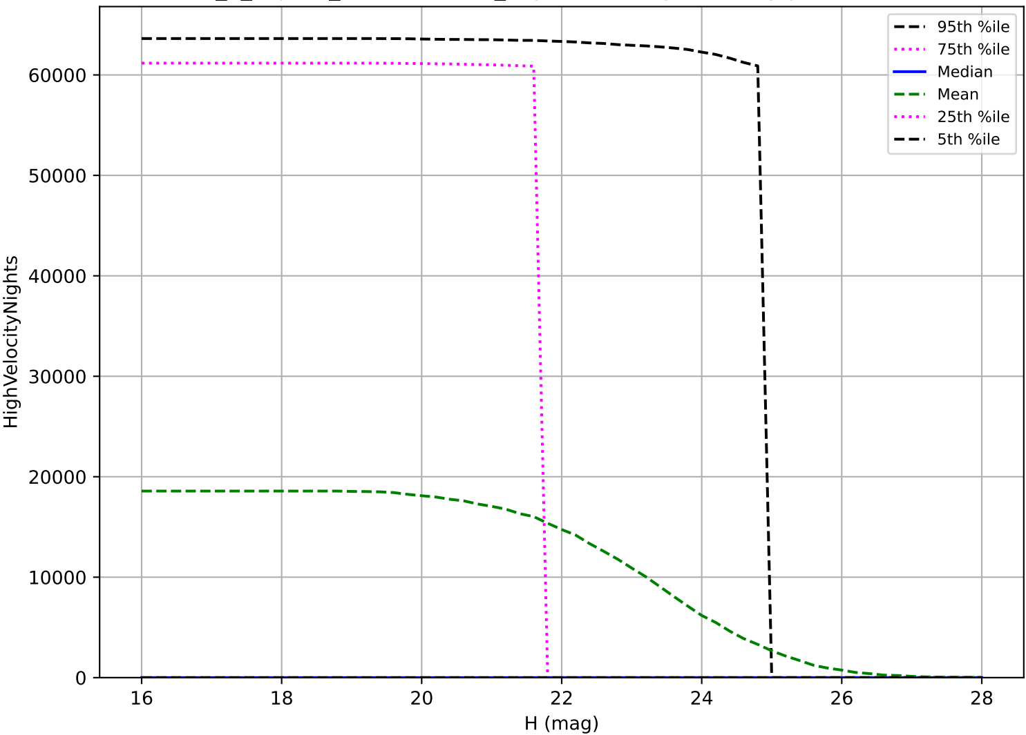
internal_u_expt30_nscale1.1v3.4_10yrs: NEO High velocity pair detection loss
