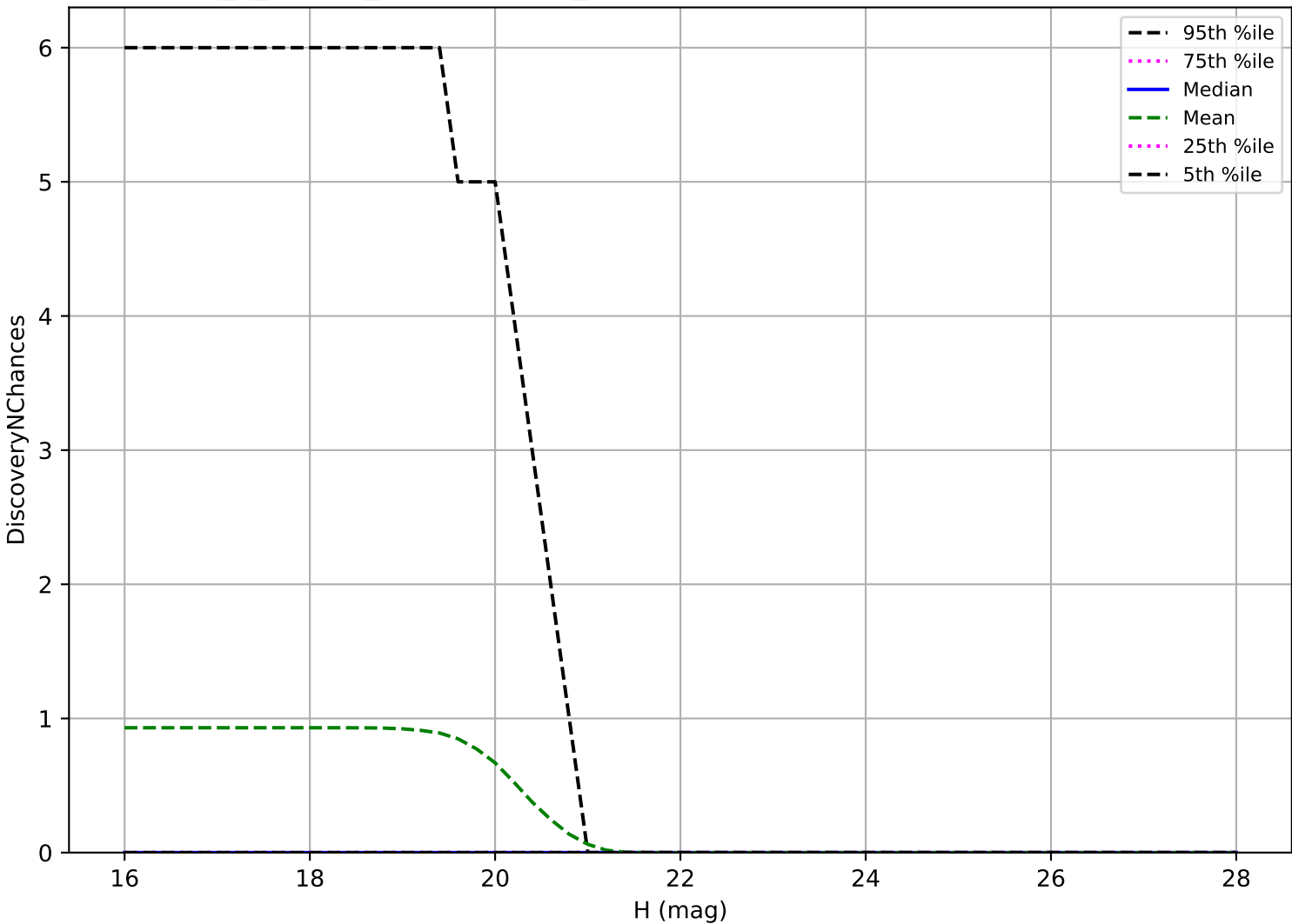
internal_u_expt30_nscale1.1v3.4_10yrs: Vatira 3 pairs in 15 nights detection loss
