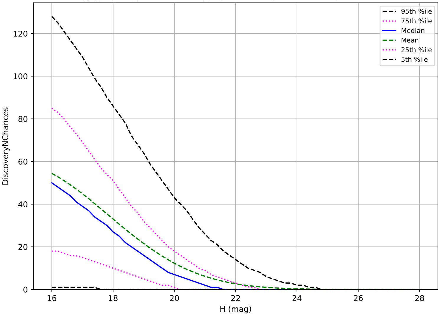
internal_u_expt30_nscale1.1v3.4_10yrs: PHA 3 pairs in 15 nights detection loss
