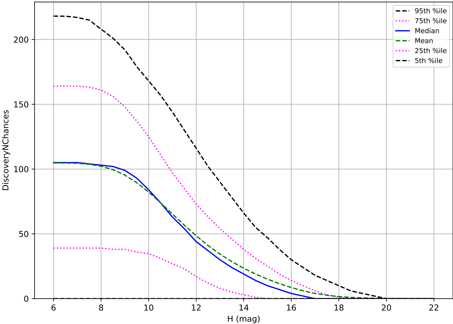
internal_u_expt30_nscale1.1v3.4_10yrs: OCC_r5 3 pairs in 15 nights detection loss
