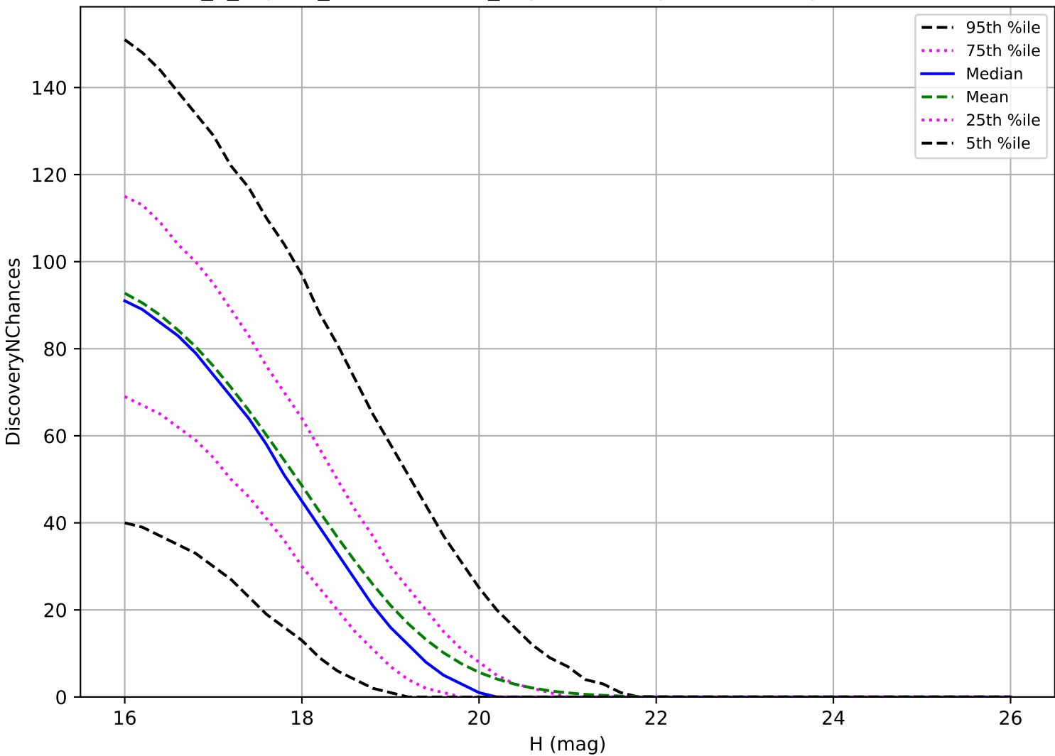
internal_u_expt30_nscale1.1v3.4_10yrs: MBA 3 pairs in 15 nights detection loss
