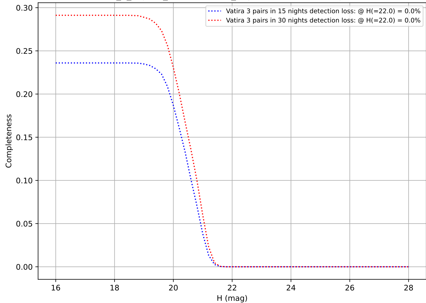
internal_u_expt30_nscale1.1v3.4_10yrs: DifferentialCompleteness
