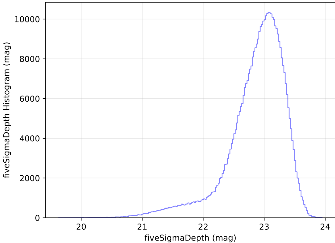
internal_u_expt30_nscale1.1v3.4_10yrs z: fiveSigmaDepth Histogram
