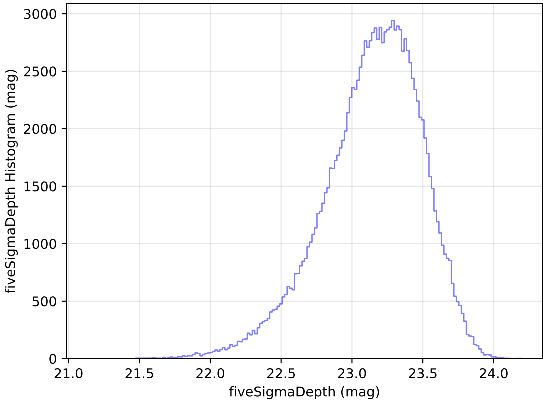
internal_u_expt30_nscale1.1v3.4_10yrs u: fiveSigmaDepth Histogram
