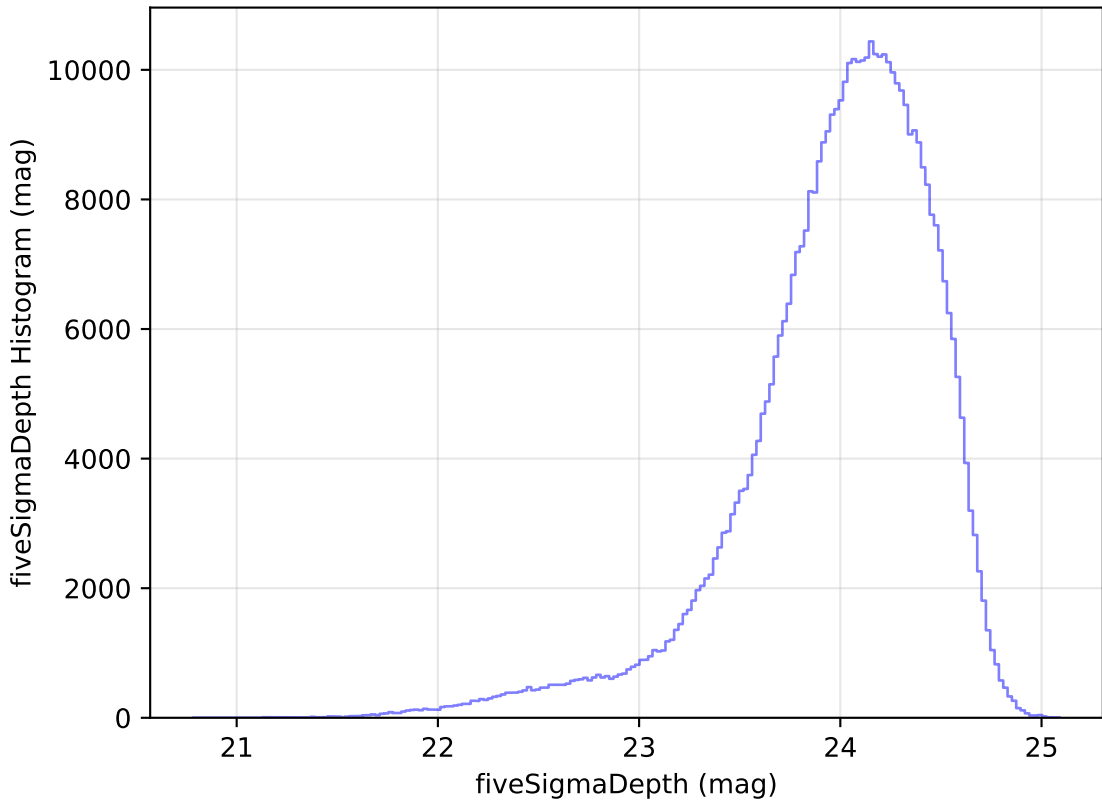
internal_u_expt30_nscale1.1v3.4_10yrs r: fiveSigmaDepth Histogram
