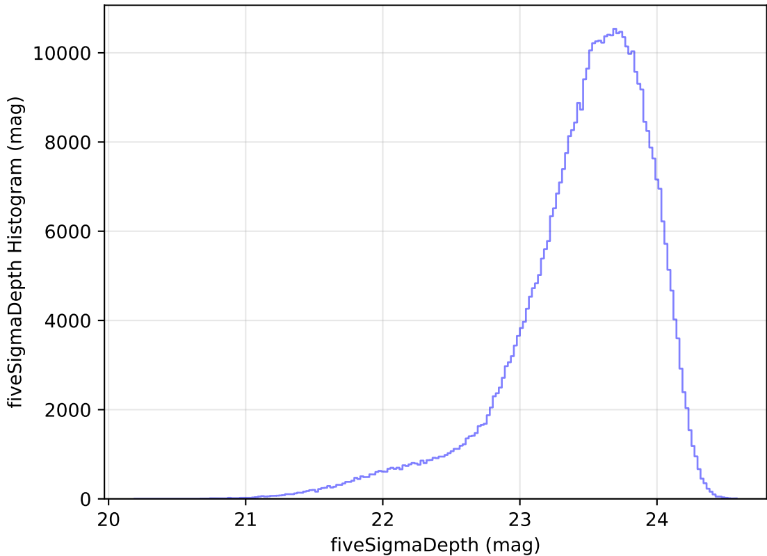
internal_u_expt30_nscale1.1v3.4_10yrs i: fiveSigmaDepth Histogram
