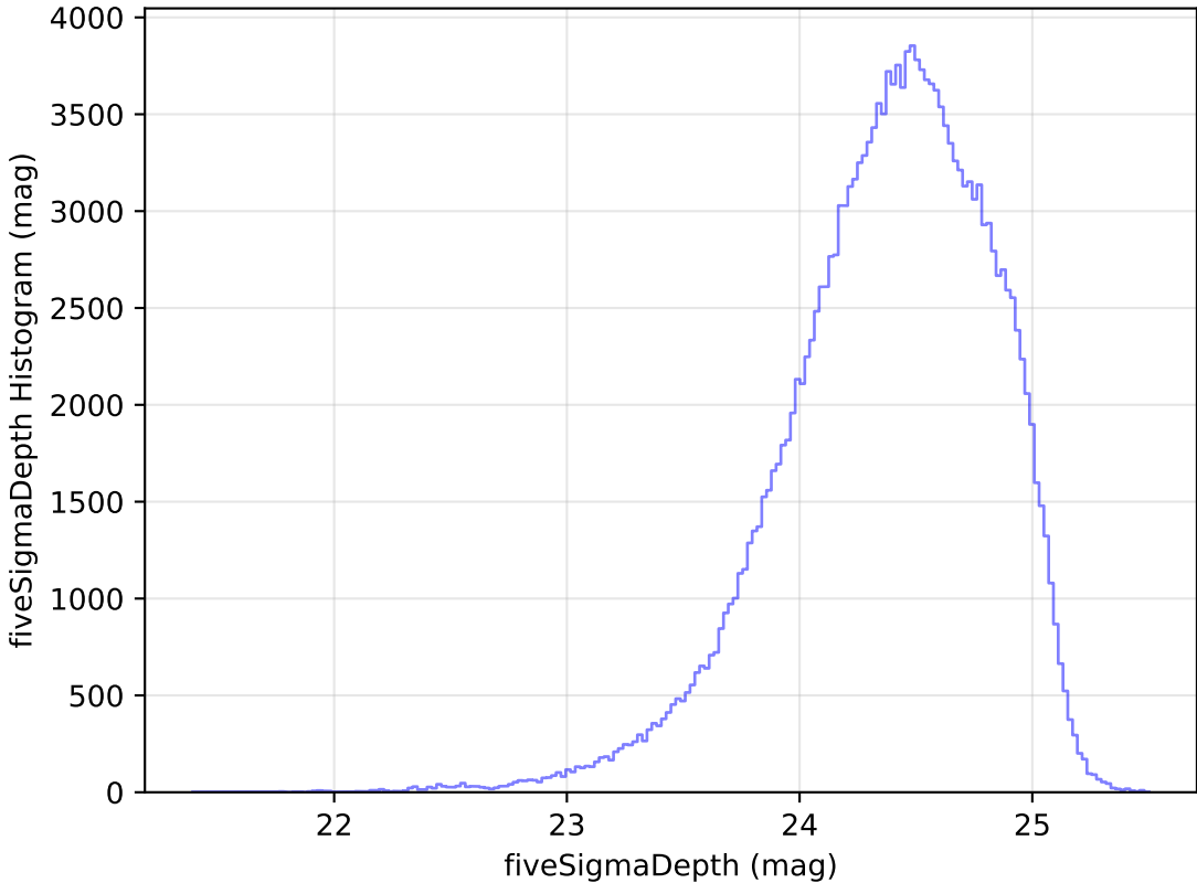
internal_u_expt30_nscale1.1v3.4_10yrs g: fiveSigmaDepth Histogram
