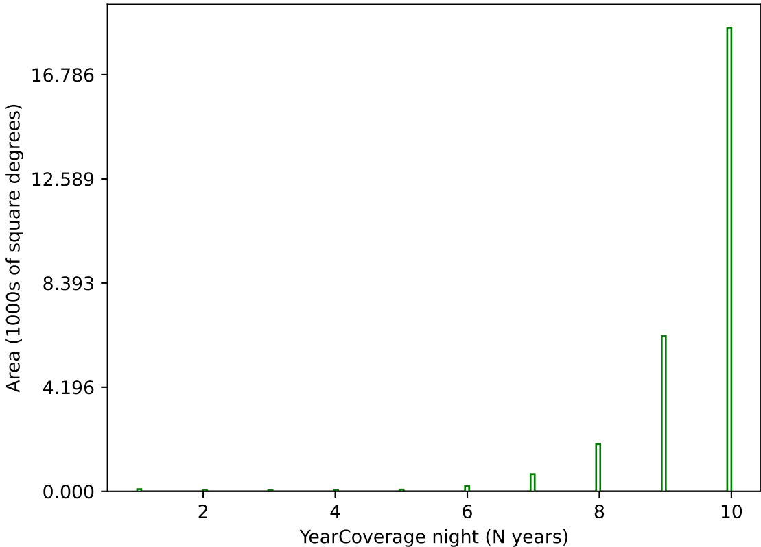
internal_u_expt30_nscale1.1v3.4_10yrs g band: YearCoverage night
