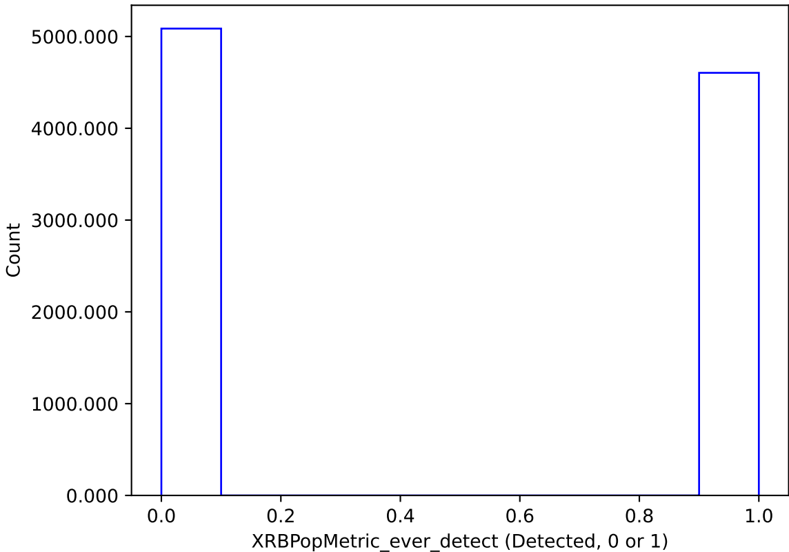
internal_u_expt30_nscale1.1v3.4_10yrs : XRBPoMetric_ever_detect
