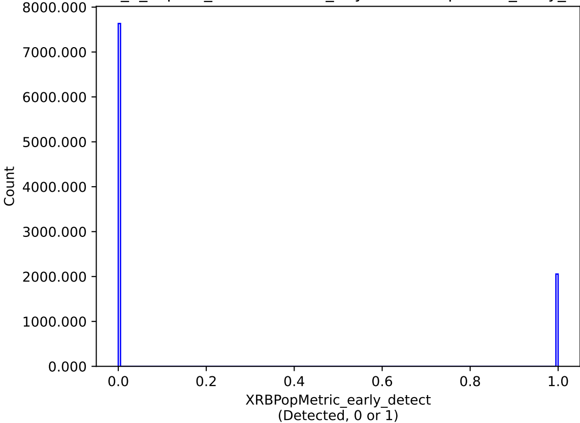
internal_u_expt30_nscale1.1v3.4_10yrs : XRBPoMetric_early_detect
