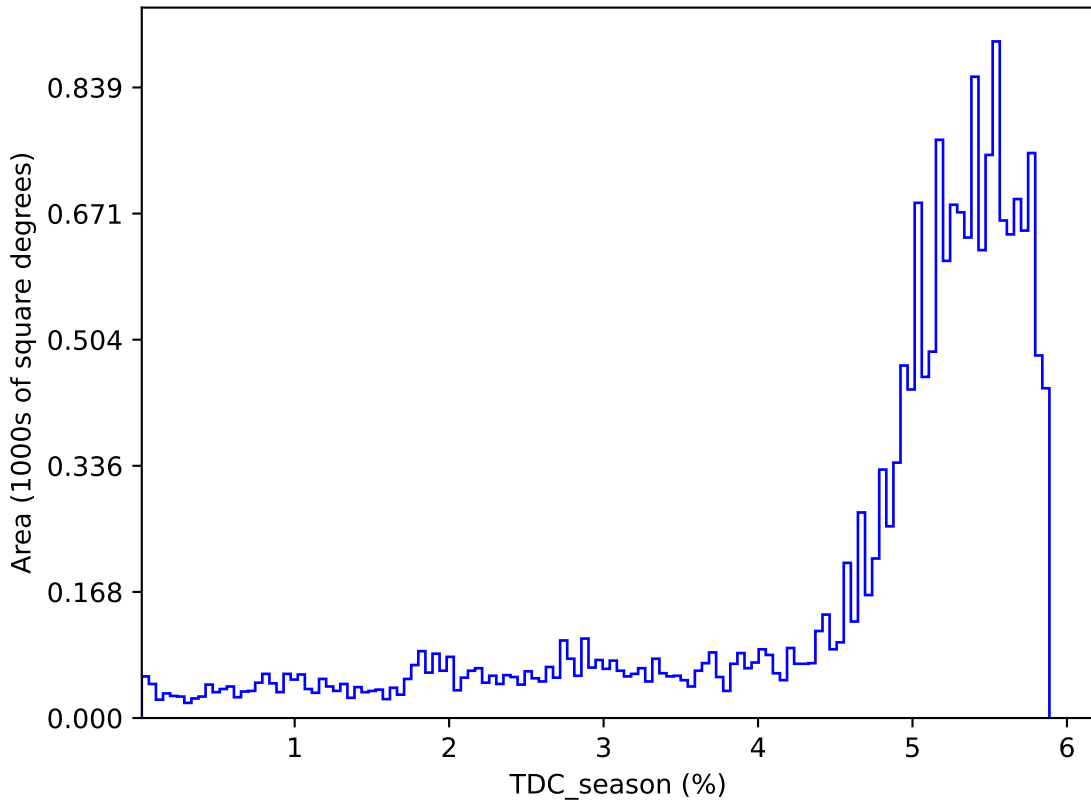
internal_u_expt30_nscale1.1v3.4_10yrs : TDC_season
