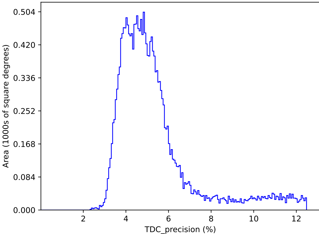
internal_u_expt30_nscale1.1v3.4_10yrs : TDC_precision
