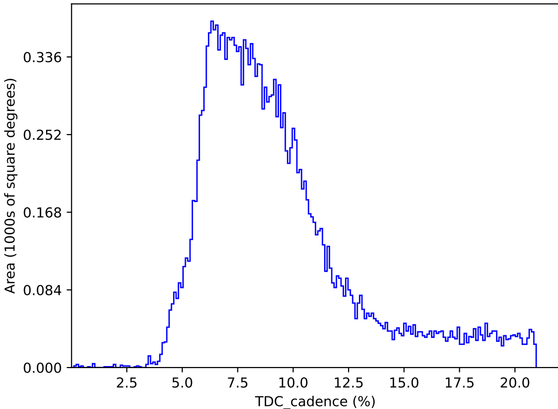
internal_u_expt30_nscale1.1v3.4_10yrs : TDC_cadence
