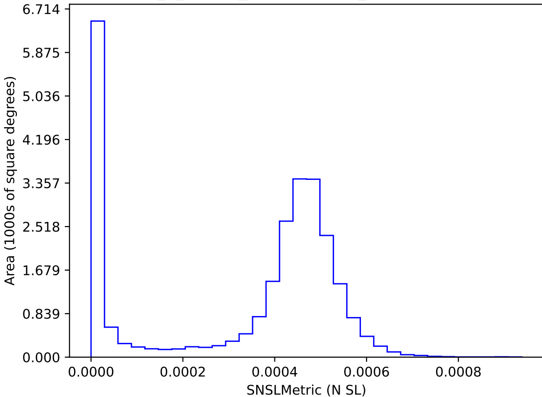
internal_u_expt30_nscale1.1v3.4_10yrs : SNSLMetric
