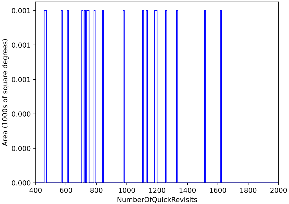
internal_u_expt30_nscale1.1v3.4_10yrs : NumberOfQuickRevisits
