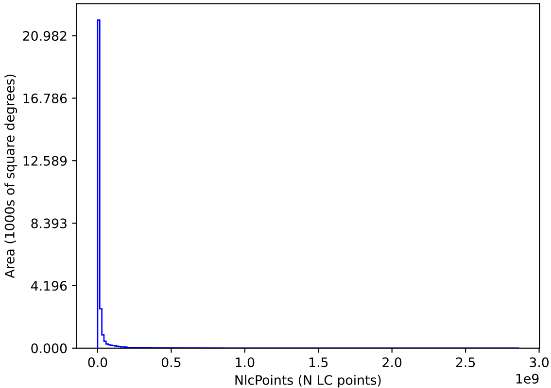
internal_u_expt30_nscale1.1v3.4_10yrs : NlcPoints
