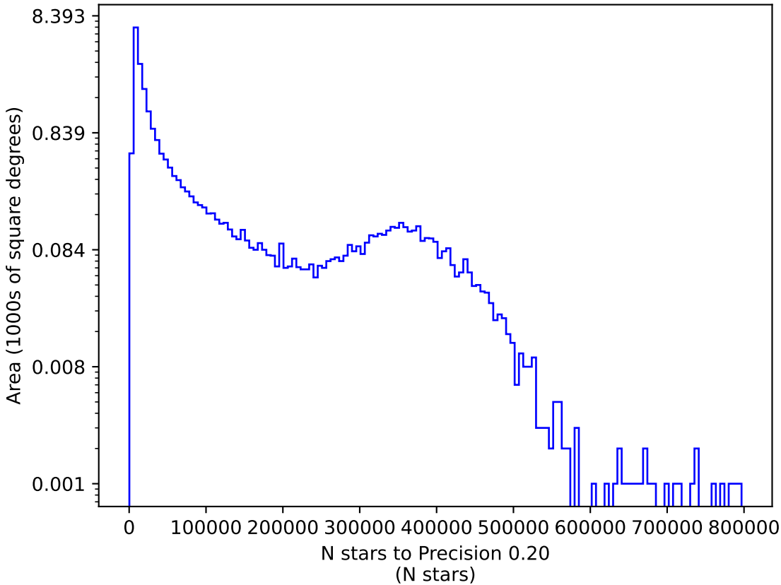
internal_u_expt30_nscale1.1v3.4_10yrs y: N stars to Precision 0.20
