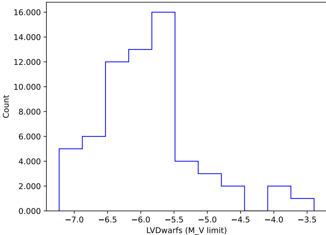
internal_u_expt30_nscale1.1v3.4_10yrs gi: LVDwarfs
