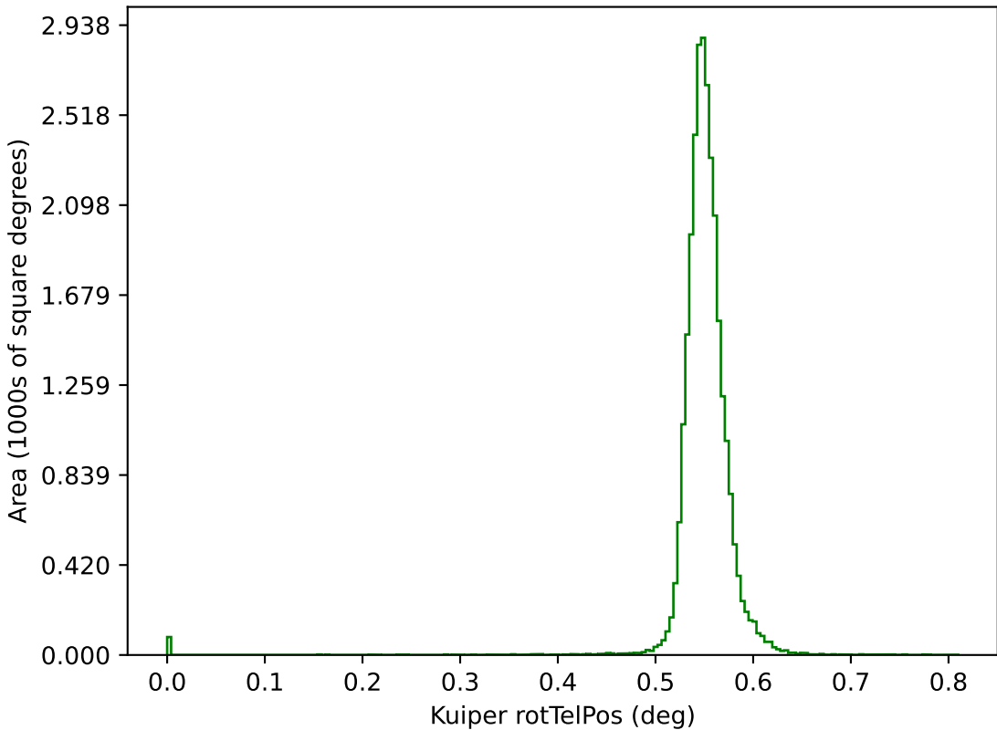
internal_u_expt30_nscale1.1v3.4_10yrs g: Kuiper rotTelPos
