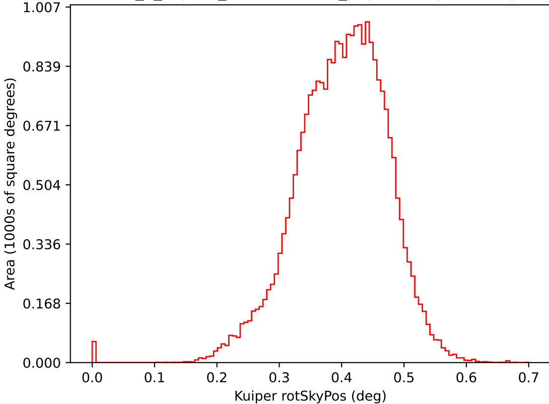
internal_u_expt30_nscale1.1v3.4_10yrs i: Kuiper rotSkyPos
